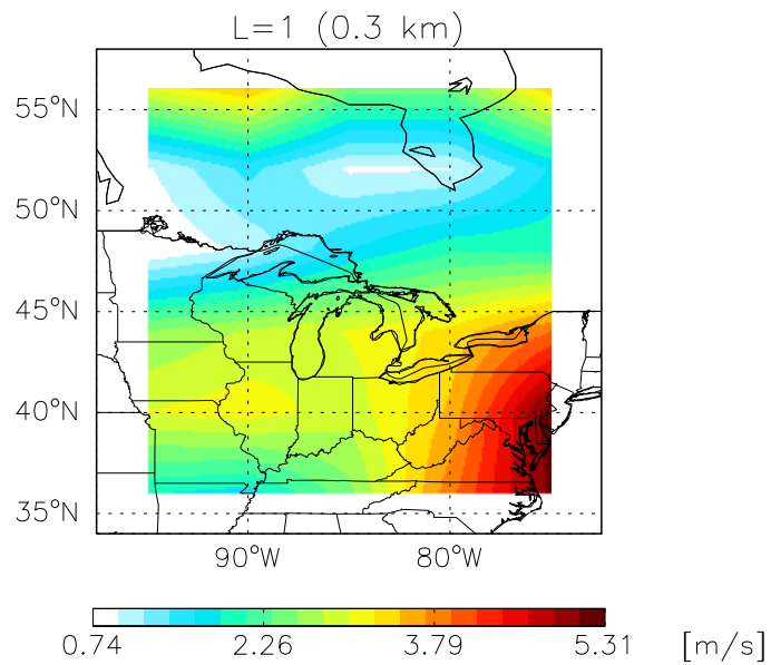
GCAP UWND Feb 1999 – Feb 2001
