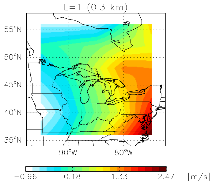
GCAP UWND Apr 1999 – Apr 2001
