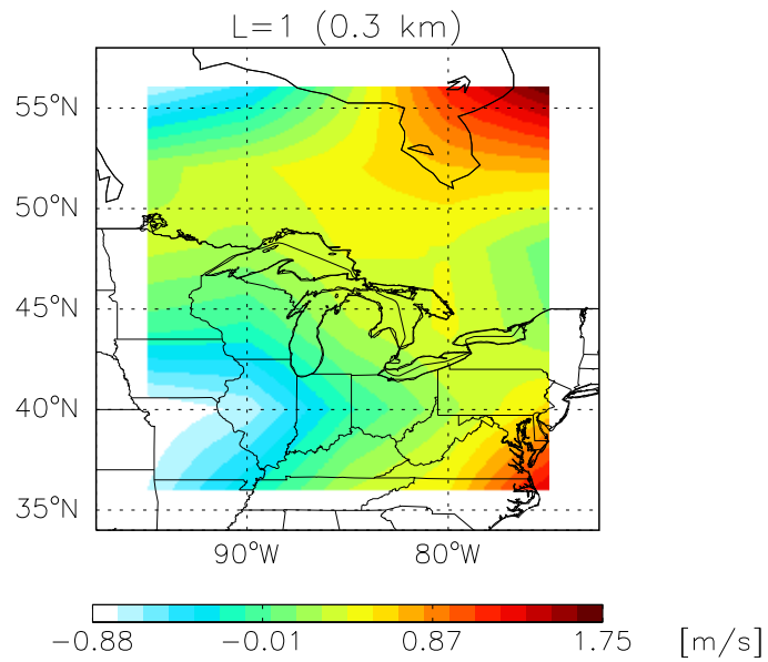
GCAP UWND Jul 1999 – Jul 2001
