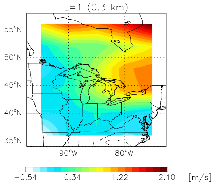
GCAP UWND Aug 1999 – Aug 2001
