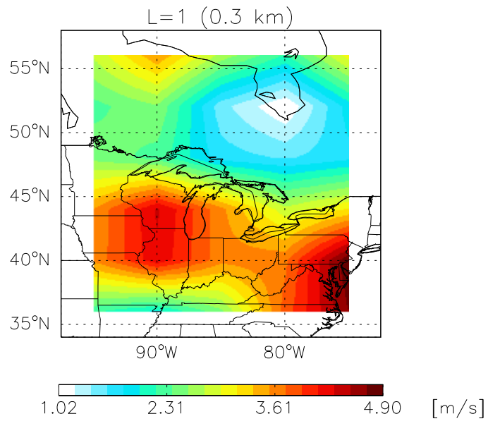
GCAP UWND Dec 1999 – Dec 2001
