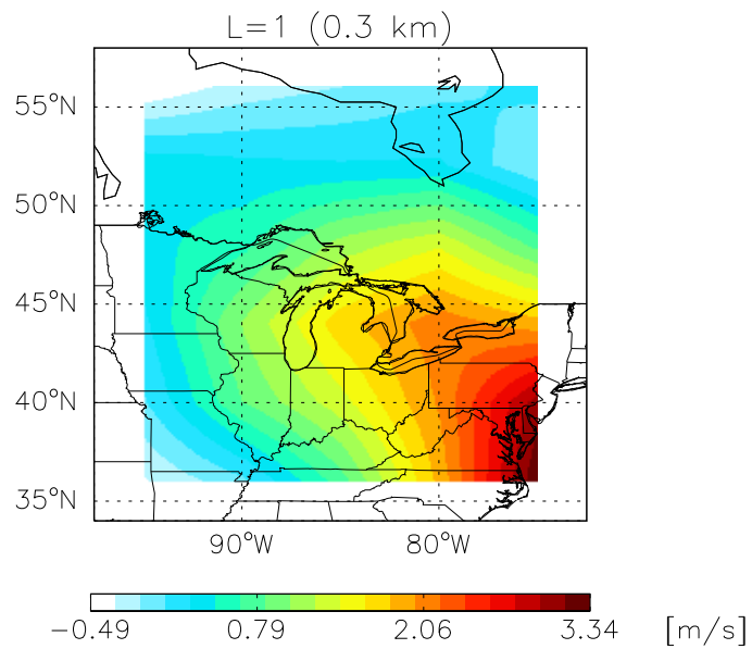
GCAP UWND May 1999 – May 2001
