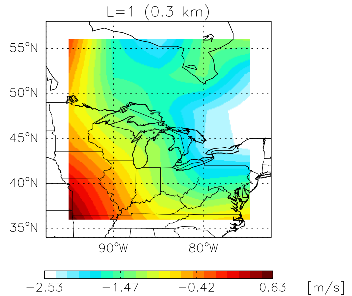
GCAP VWND Apr 1999 – Apr 2001
