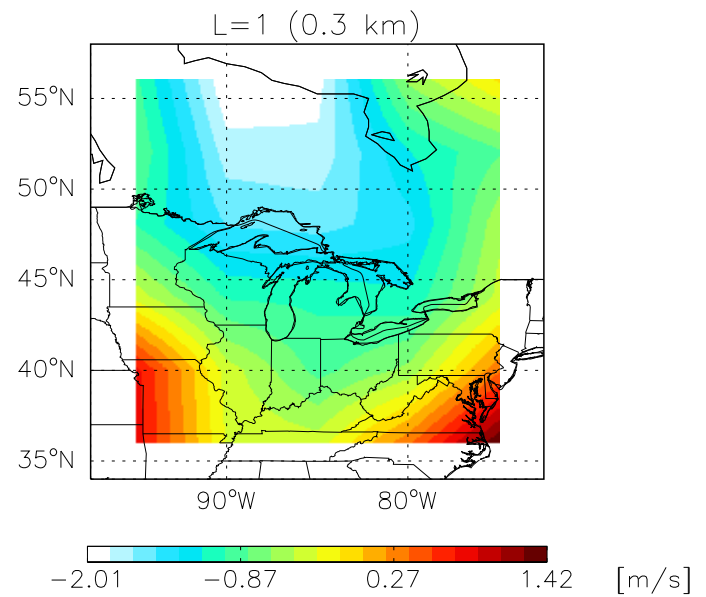
GCAP VWND May 1999 – May 2001
