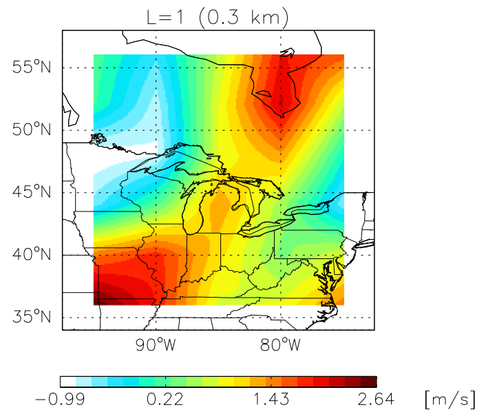
GCAP VWND Jan 1999 – Jan 2001
