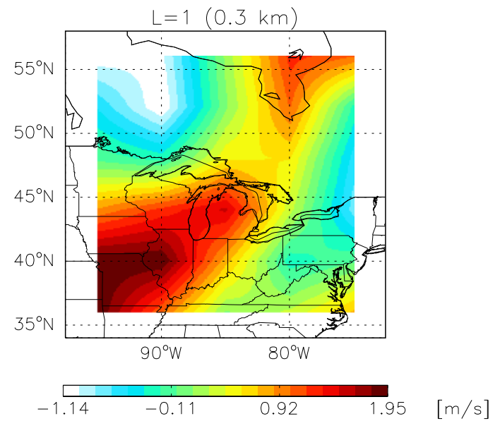
GCAP VWND Feb 1999 – Feb 2001
