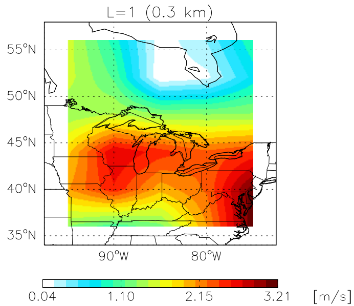
GCAP UWND Nov 1999 – Nov 2001
