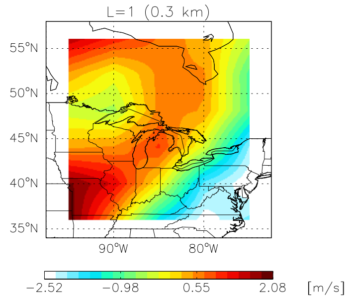
GCAP VWND Nov 1999 – Nov 2001
