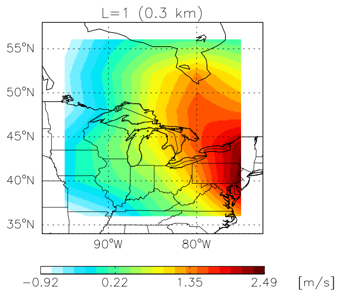
GCAP UWND Jun 1999 – Jun 2001
