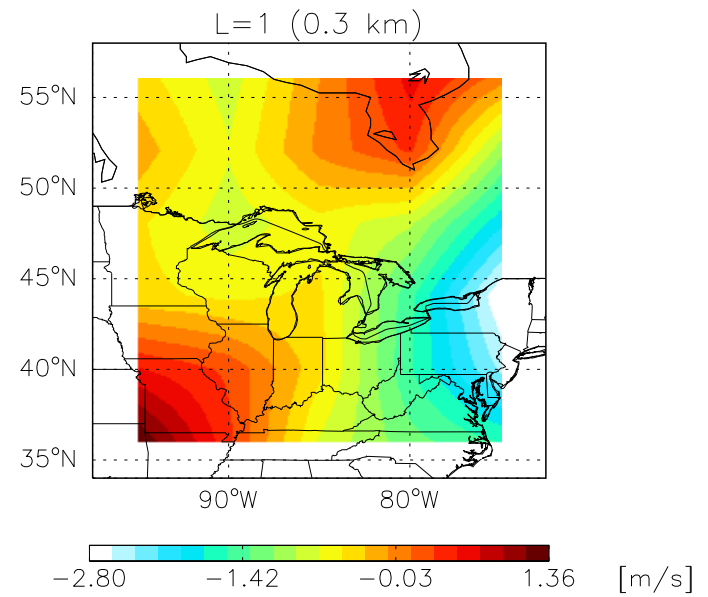
GCAP VWND Mar 1999 – Mar 2001
