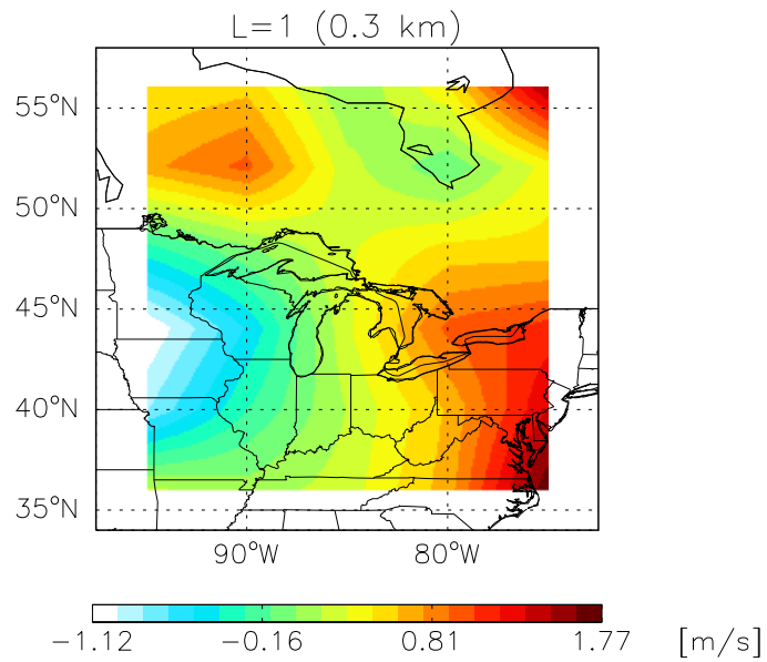
GCAP UWND Mar 1999 – Mar 2001
