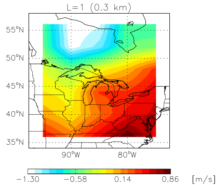
GCAP VWND Aug 1999 – Aug 2001
