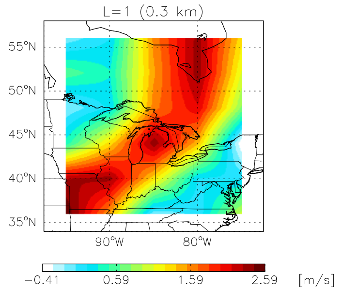
GCAP VWND Dec 1999 – Dec 2001
