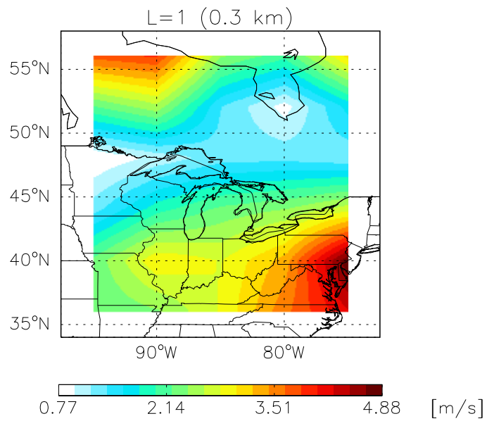
GCAP UWND Jan 1999 – Jan 2001
